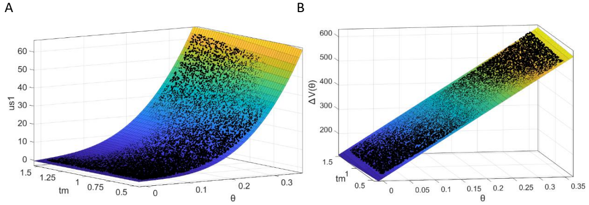
Fig. S4. Surface fitting visualization. (A) The fitted result of the integrand corresponding to the integral function U_{s1}(\theta) , R-square: 0.9999, RMSE:0.1572; (B) The fitted result of the integrand corresponding to the integral function \Delta V(\theta) , R-square: 0.9999, RMSE: 0.8883.
