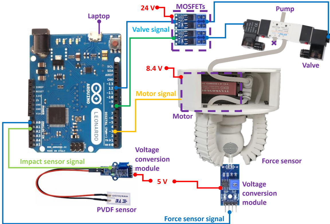
Fig. S8. The control system scheme.
