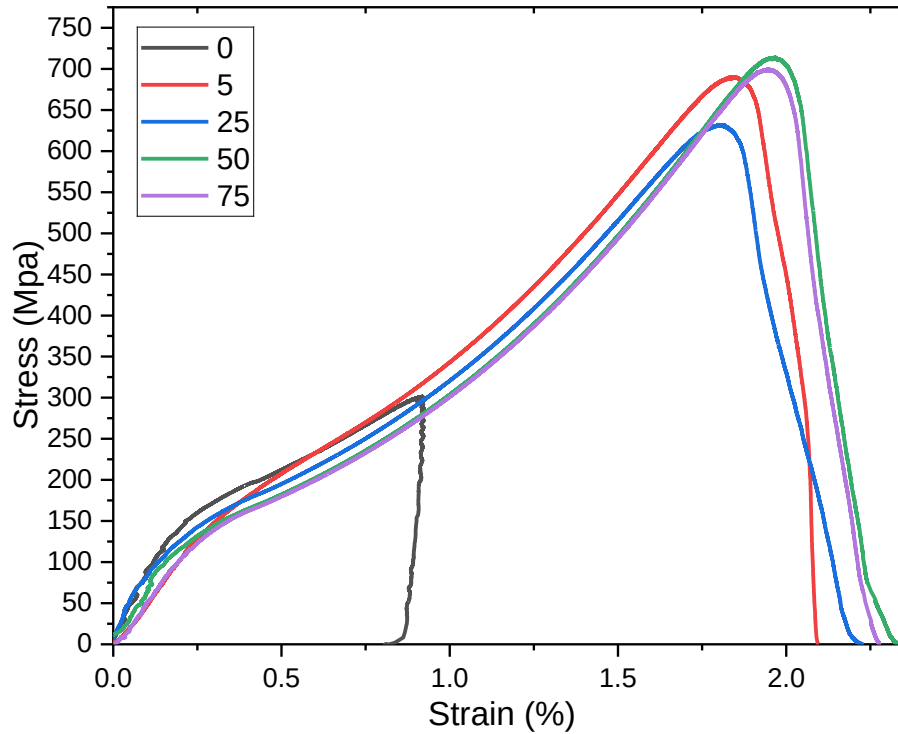
Fig. S3. The result of the tensile test with different numbers of bending cycles.
