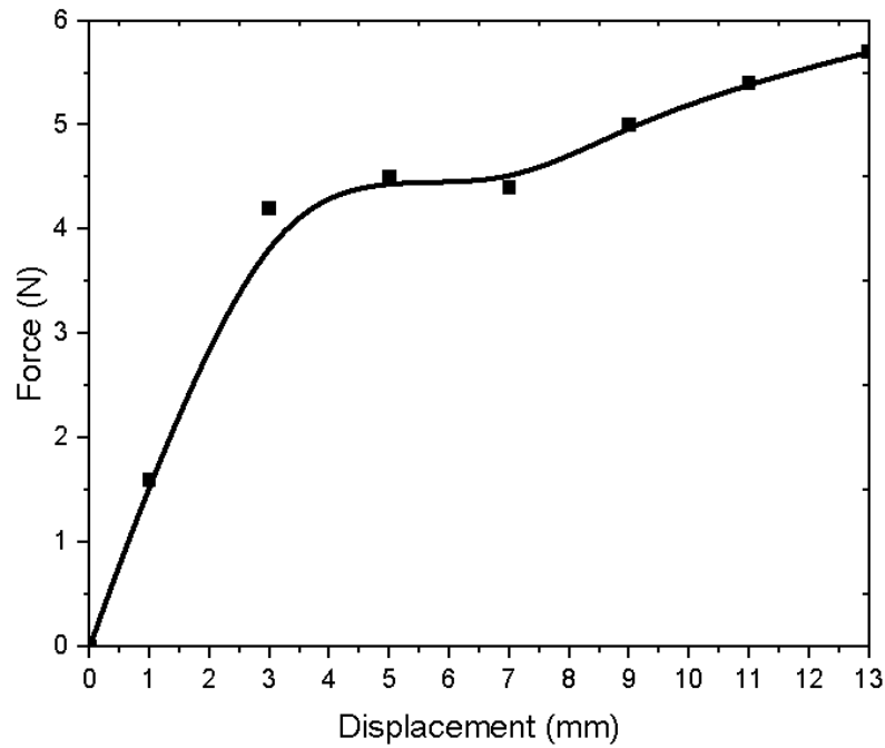
Fig. S2. Force-displacement characteristics of the paw pad. The sensor exhibits high sensitivity to external forces at the initial stage of displacement, allowing for enhanced detection of object contact. When the displacement exceeds approximately 4 mm, the sensitivity decreases, indicating a transition to a stable support phase that provides a consistent supporting force of around 4.5 N for the grasped object.
