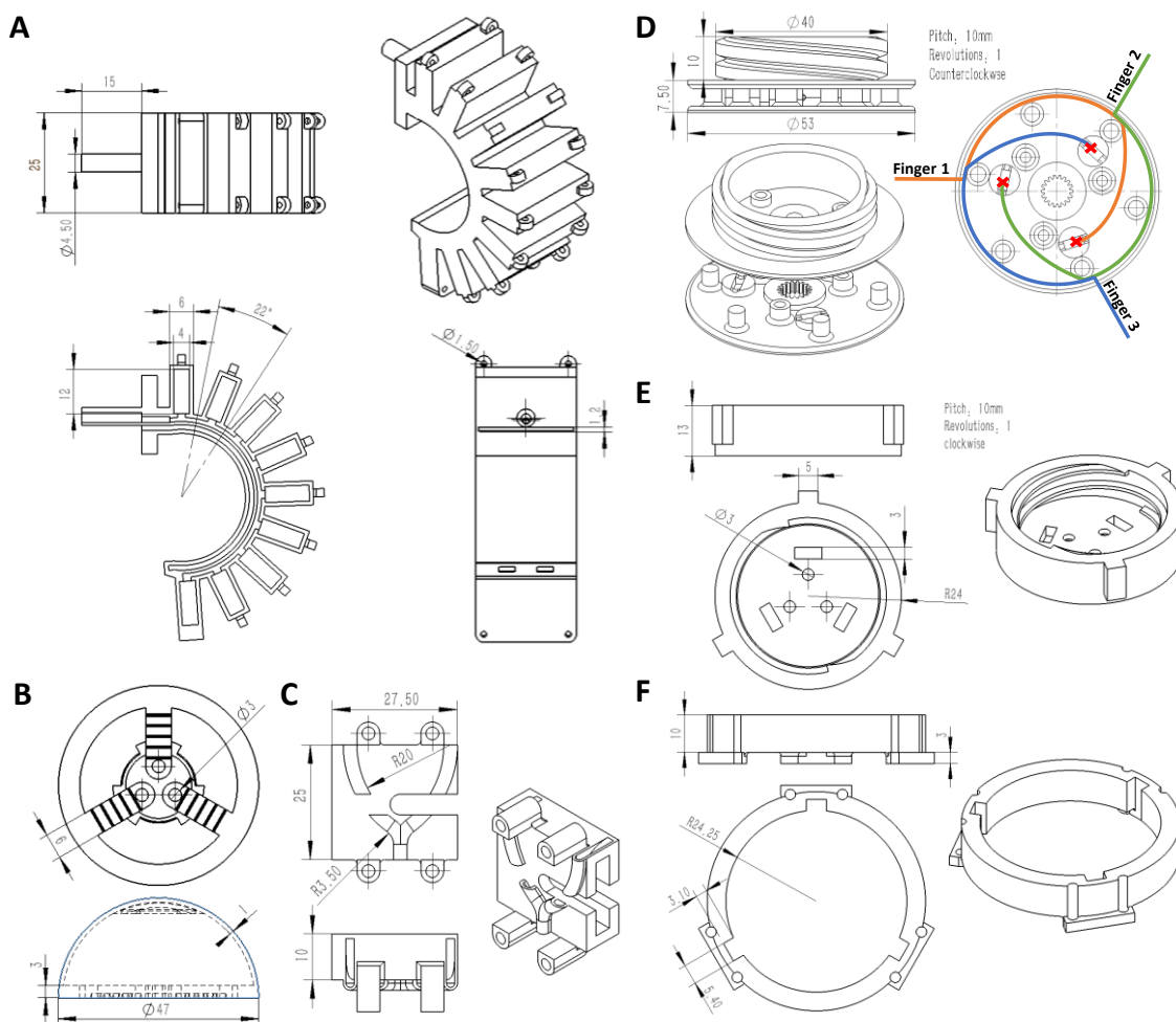
Fig. S1. Schematic representation of the component dimensions. (A) Soft finger; (B) Paw pad; (C) Soft finger fixture; (D) Screw; (E) Flanged nut; (F) Linear guide. Due to the thermoplastic effect of TPU, the initial angle of the soft finger 3D printed will be smaller than the set pre-stretching angle.
