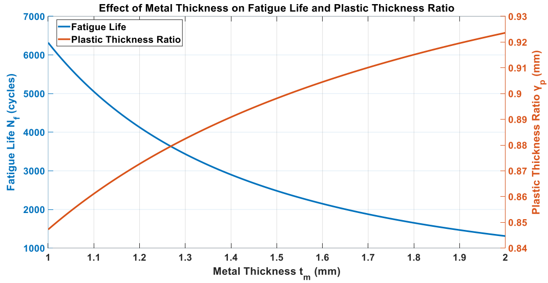
Fig. S10. Effect of metal-layer thickness on fatigue life and plastic deformation behavior.
