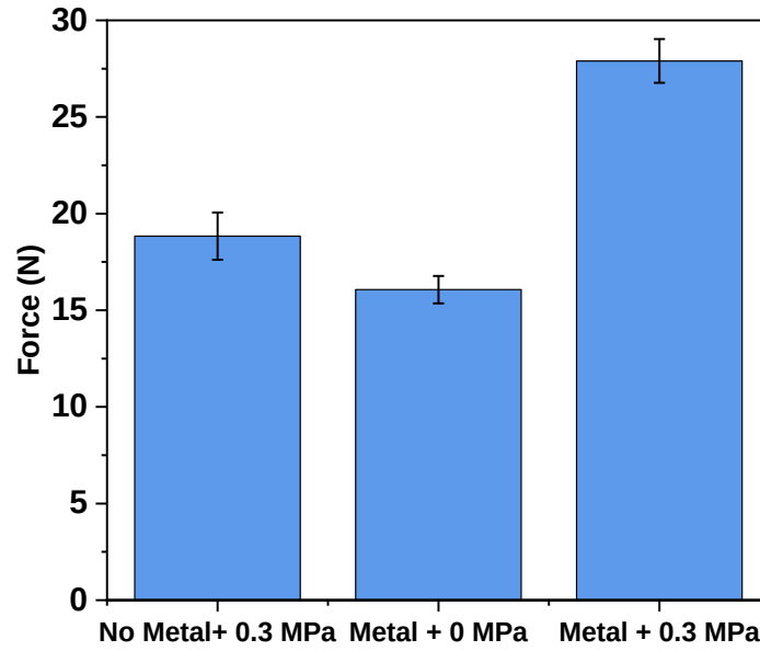
Fig. S6. Static stability experiments results. The experiments were performed by grasping a 150 g ball-shaped object with an internal iron core, and a vertical downward force was applied using a digital force gauge to measure the maximum load the gripper could resist in a static state. For each condition, the maximum holding force in the static condition was measured three times.
