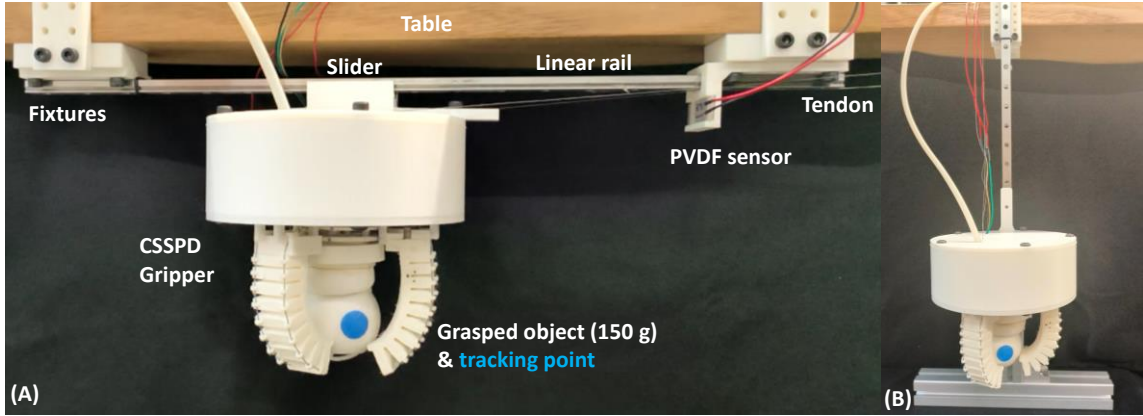
Fig. S9. Experimental setup. (A) Horizontal stability test platform. (B) Vertical stability test platform. The impact force F and impact duration \Delta t can be obtained using the PVDF sensor. Due to the high sensitivity of the PVDF sensor, the measured impact time is very short, averaging around 10 ms. Therefore, the measured force can be regarded as the actual instantaneous force during the impact, and the resulting acceleration can be calculated using a = F/m .
